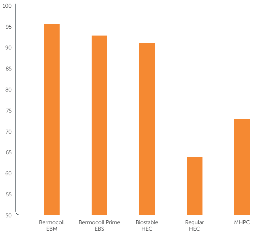
Enzyme resistance Retained viscosity in %
